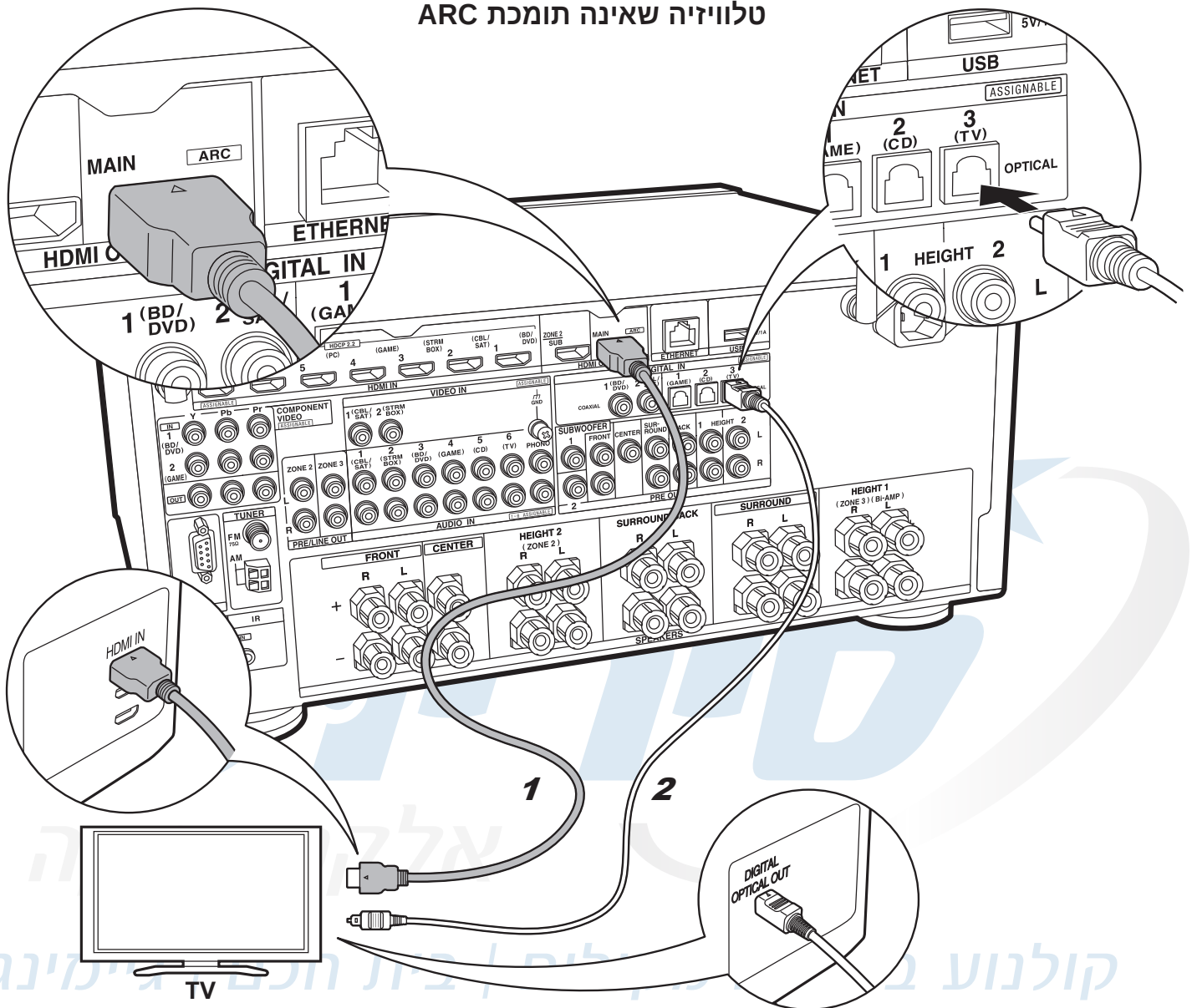
1 HDMI cable, 2 Digital optical cable
