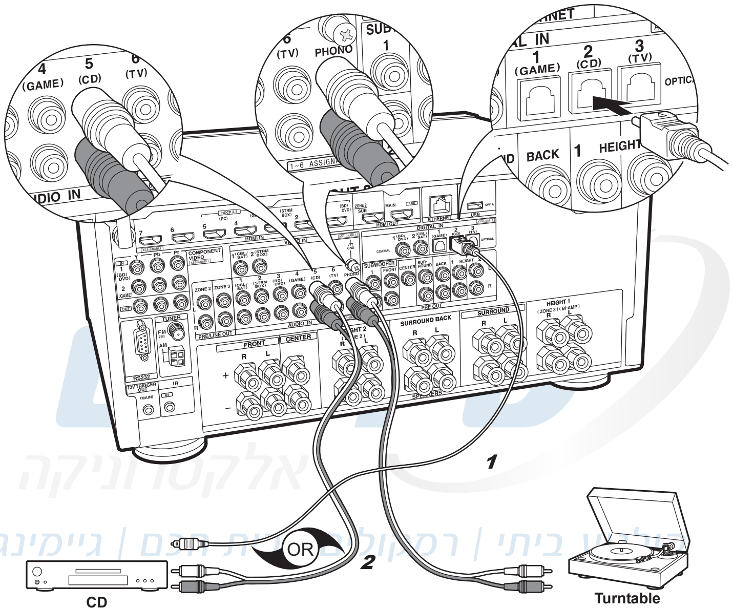
1 Digital optical cable, 2 Analog audio cable
