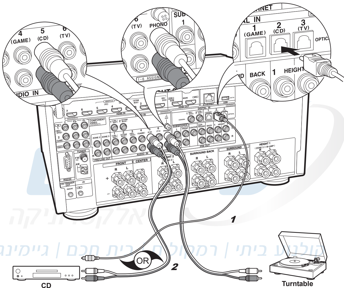
1 Digital optical cable, 2 Analog audio cable
