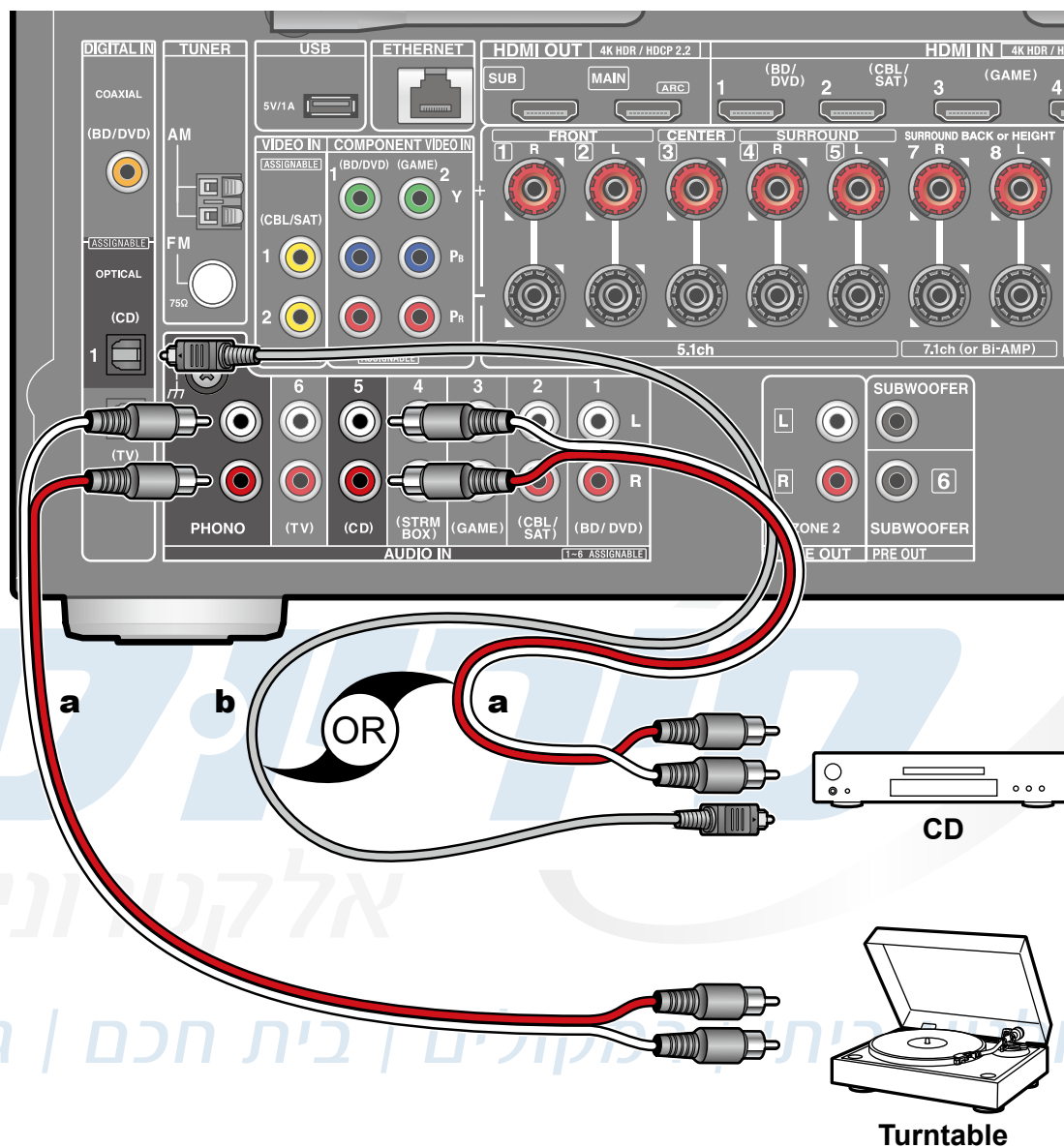
a Analog audio cable , b Digital optical cable
